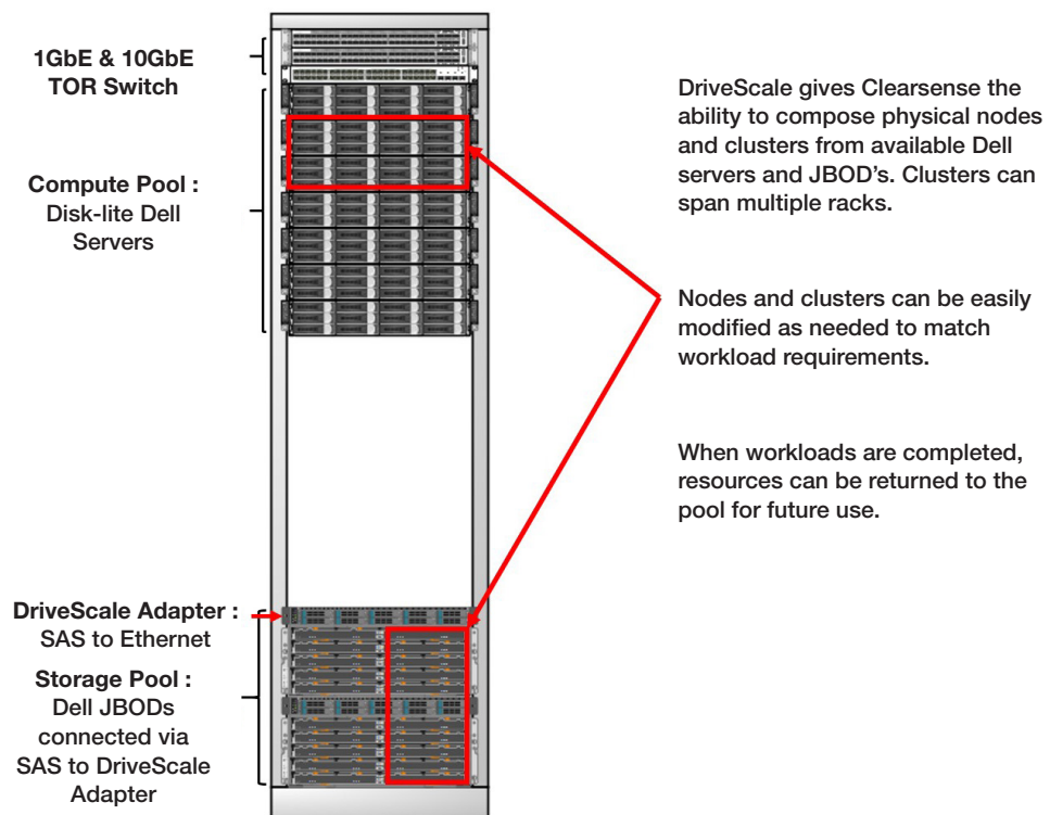
Figure 1: Illustration of DriveScale SCI architecture
